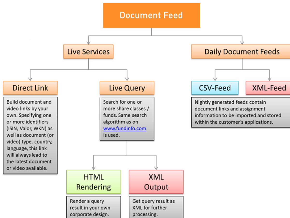
Fig. 1: Document Feed services
